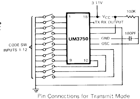
Pin Connections for Transmit Mode
